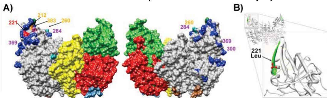
Fig. 4. The TfR structure, based on a model of the human receptor (domains are colored on one monomer – protease-like = red, apical = green, helical = yellow). Residues tested for effects on the binding of CPV are colored: no clear effect on virus binding dark blue, alteration of virus binding red or purple. Known Asn-linked glycosylation sites labeled in orange. A portion of the stalk domain is colored in cyan (left), and transferrin binding sites are brown (right). B) The position of residue Leu 221 in the apical domain.
