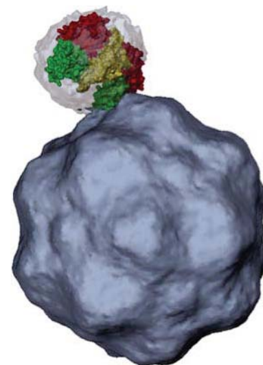
Fig. 5. The cryoEM structure of the feline TfR in complex with the CPV capsid.
