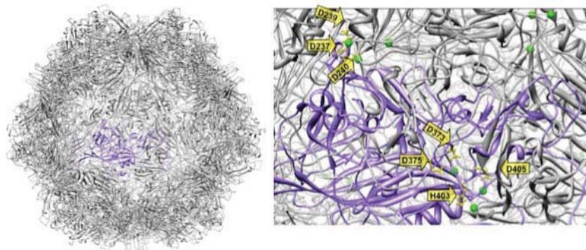
Fig. 1. The CPV capsid structure showing the position of one VP2 molecule. The blow-up shows the positions of three divalent ions (most likely \text{Ca}^{2+} ) that are bound in the structure, and the residues that coordinate them.
